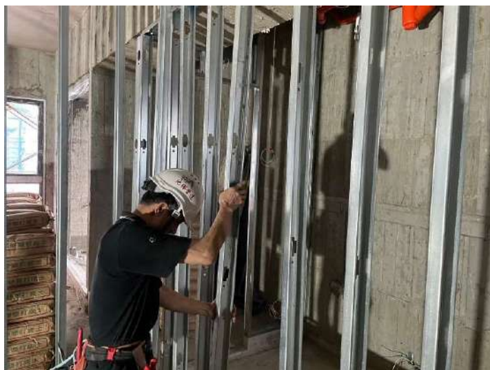
9F輕隔間骨架施作
