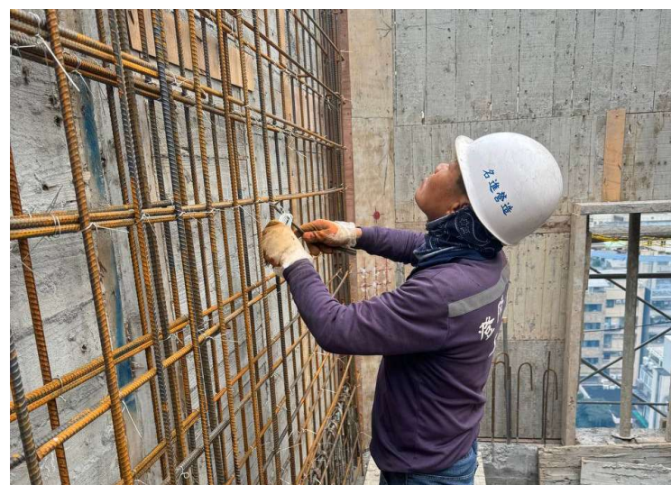
R1F 牆筋綁紮
