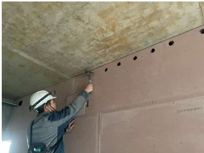
輕隔間灌漿
